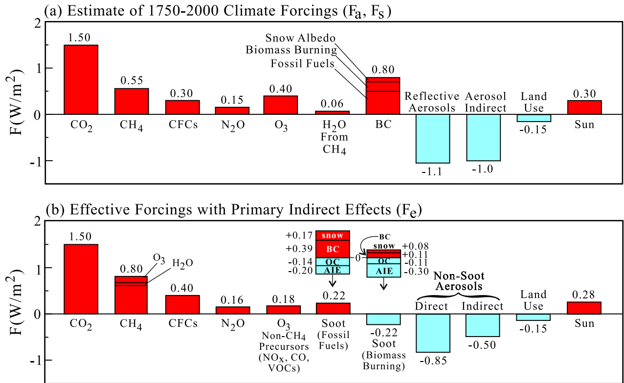
Figure 28. (a) a specific estimate of climate forcings for 1750-2000, (b) same as (a) but the effective forcings partially sorted by sources.
