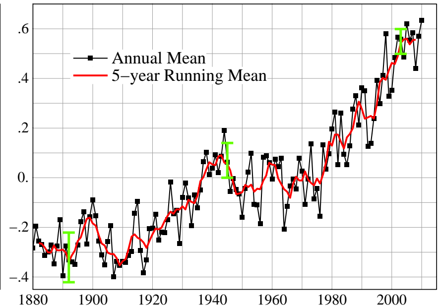
Global Land–Ocean Temperature Index with GHCN V3
