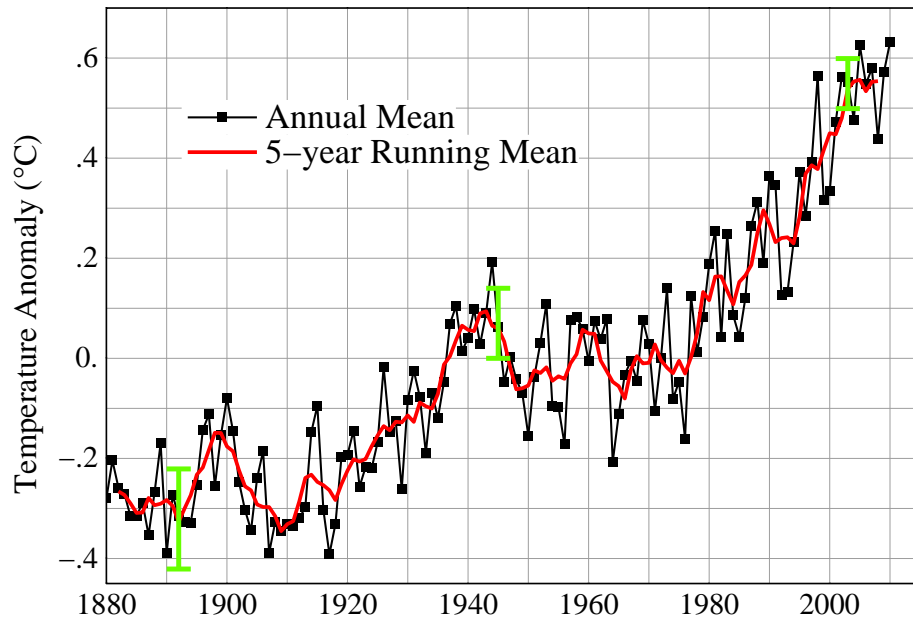
Global Land–Ocean Temperature Index with GHCN V2
