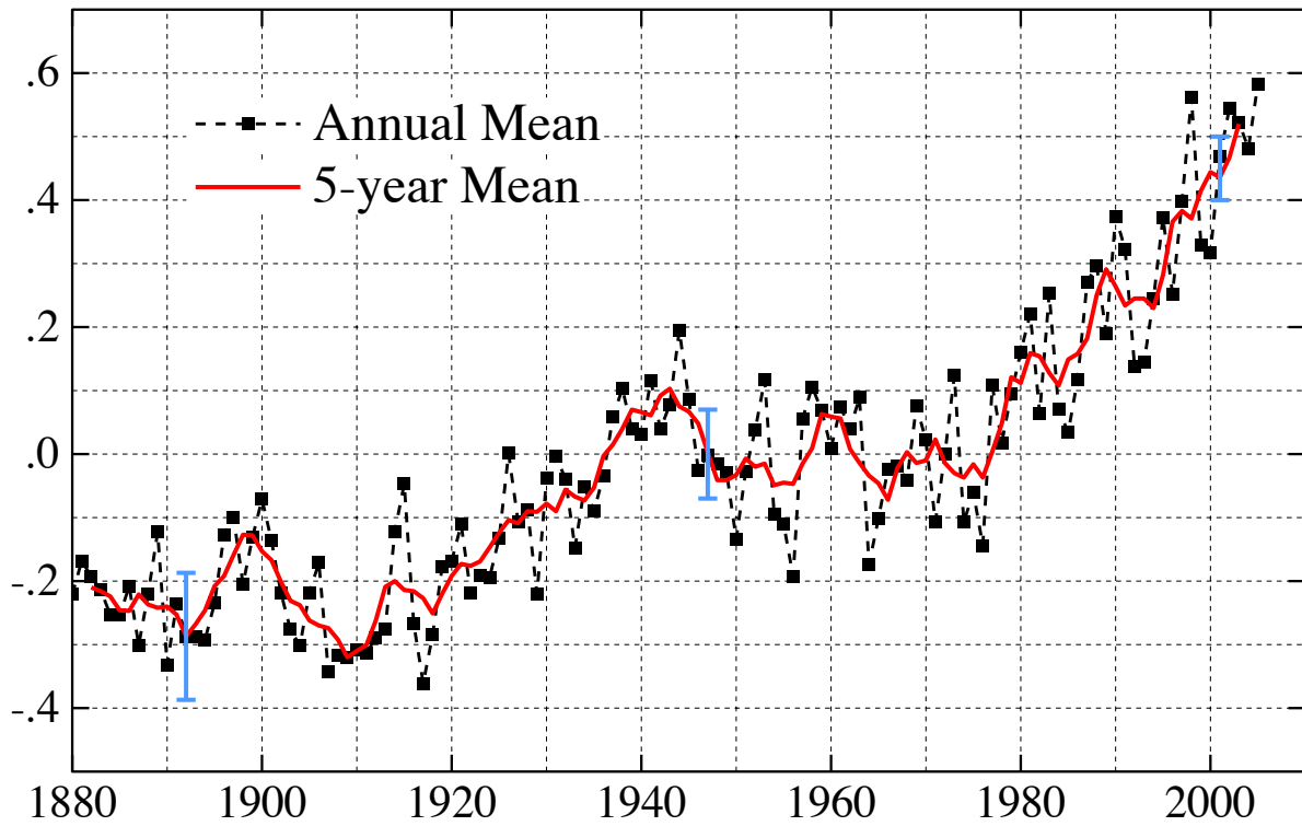
(a) Global-Mean Surface Temperature Anomaly ( ^{\circ}\text{C} )
