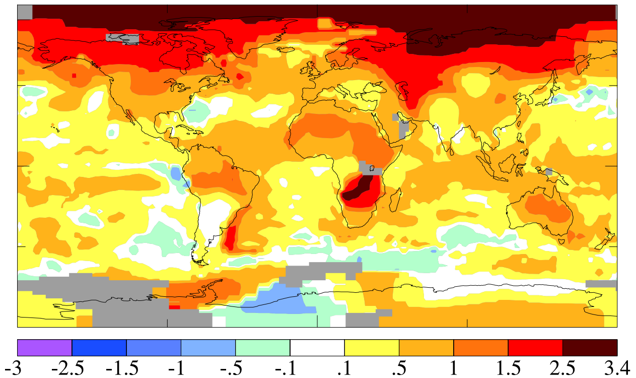
(b) 2005 Surface Temperature Anomaly ( ^{\circ}\text{C} )
